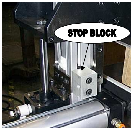
Figure 3.2 – stop block
